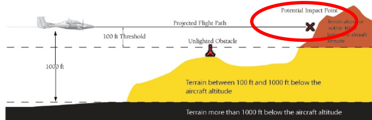
Figure 6-51 Terrain Altitude/Color Correlation for TERRAIN-SVS
