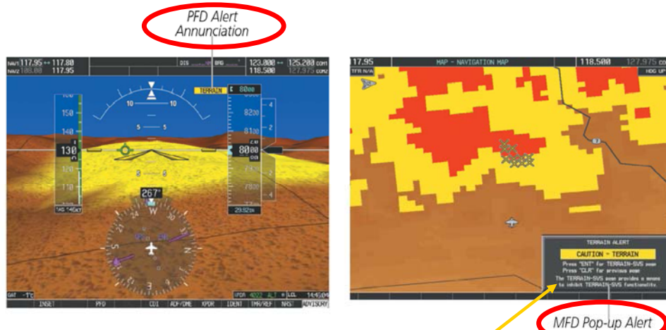
Figure 6-174 Terrain-SVS Alert Annunciations
