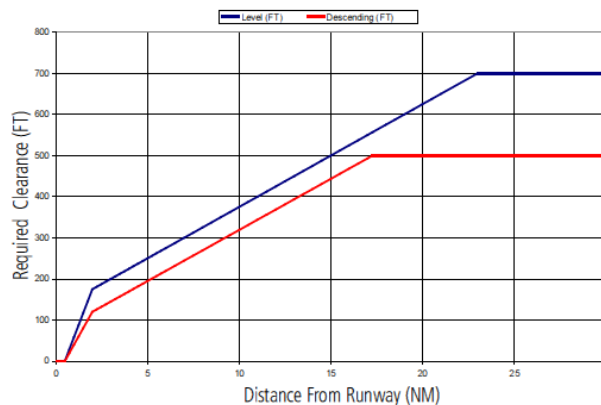
Figure 6-76 FLTA Alert Minimum Terrain and Obstacle Clearance Values
