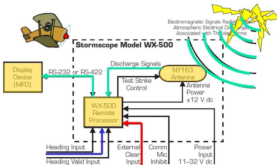
Figure 1-2. Functional Diagram
