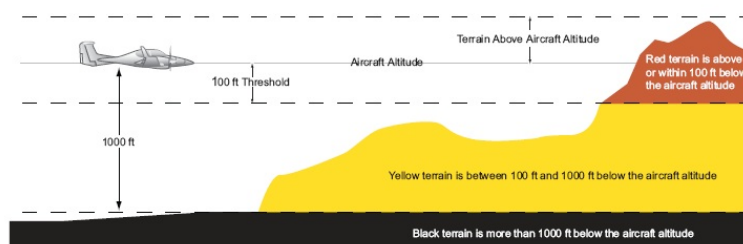
Figure 6-44 Terrain Altitude/Color Correlation for Terrain Proximity
